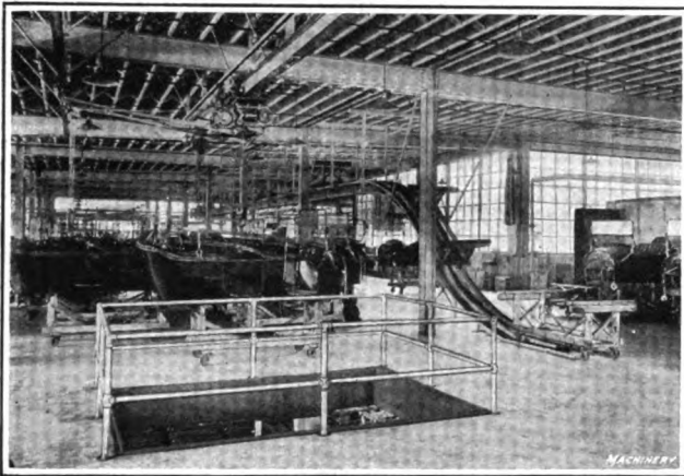
Fig. 20—Economy of space is a point of vital importance in plants handling a large volume of product. This illustration shows how automobile bodies are handled in the Willlys-Overland Co.'s plant in Toledo, O. The assembled bodies are picked up and carried away on a trolley hoist, and empty trucks are carried back to the beginning of the assembling line on the overhead track.
